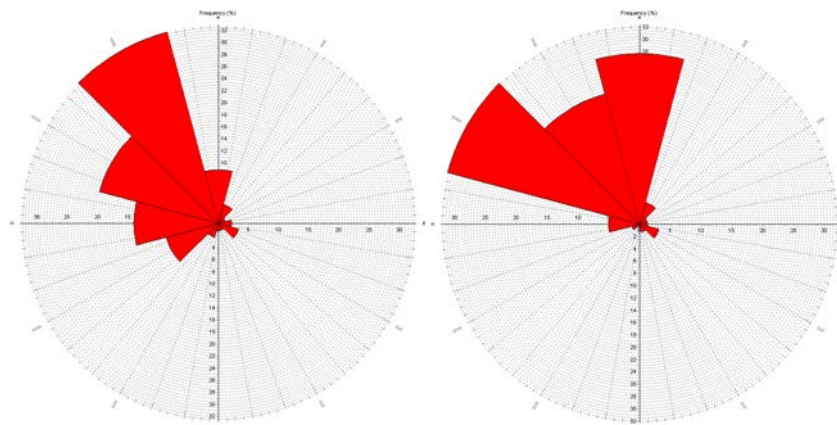
Figure 4.4: Wind rose at measurement mast and HURGHADA INTL station
