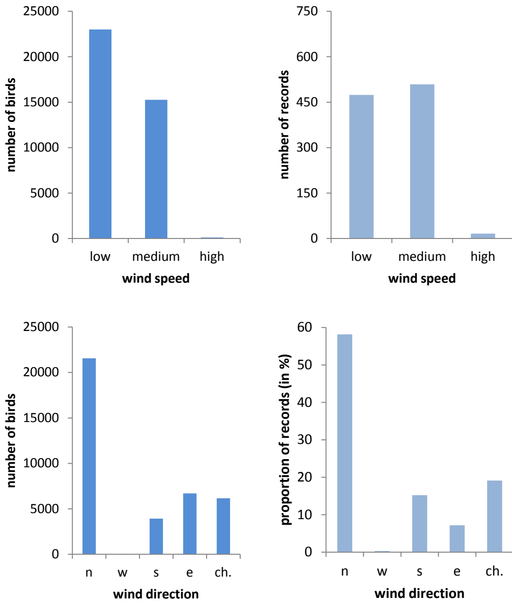
Figure 4.58: Total numbers of birds (left) and records (right) registered in the Alfancar area during certain wind speed (above) and wind direction (below) conditions in spring 2016
