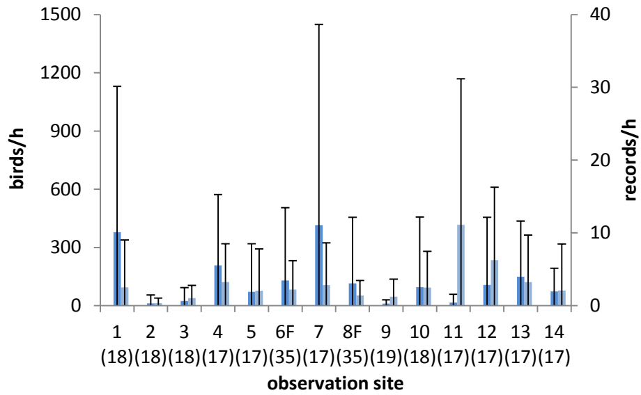
Figure 4.36: Comparison of migration rates (birds/h (blue) and records/h (light blue)) at the 14 observation sites in the study period (April 15 th to May 25 th ) in spring 2016 (arithmetic mean and standard deviation over all observation units; sample size (i.e. no. of observation units) at each observation site is given in brackets)
