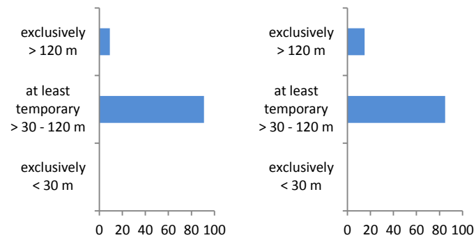
Relative abundance (percentage) of birds recorded at different altitude classes in the study area in spring 2016 (n=11; left) and 2017 (n=20; right)
