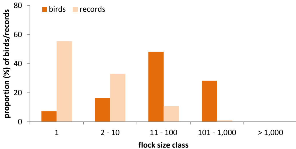
Figure 4.19: Relative abundance (proportion in %) of all birds/records registered at distances of up to 2.5 km in different flock size classes in the study period in autumn 2016
