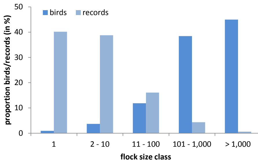
Figure 4.43: Relative abundance (proportion in %) of all birds/records registered at distances of up to 2.5 km in different flock size classes in the study period in spring 2017
