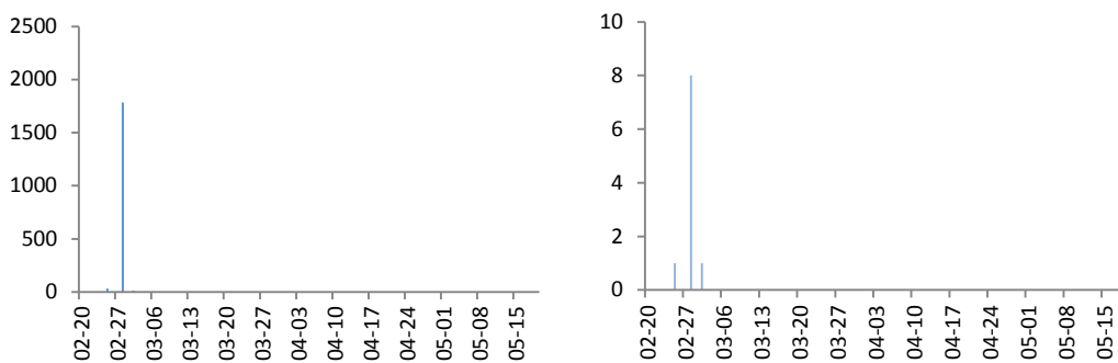
Number of birds (left) and records (right) registered in the study area in spring 2017
