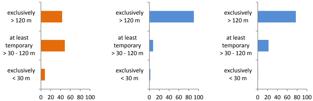
Relative abundance (percentage) of birds recorded at different altitude classes in the study area in autumn 2016 (n=37; left), spring 2016 (n=1,030; middle) and spring 2017 (n=4,077; right)
