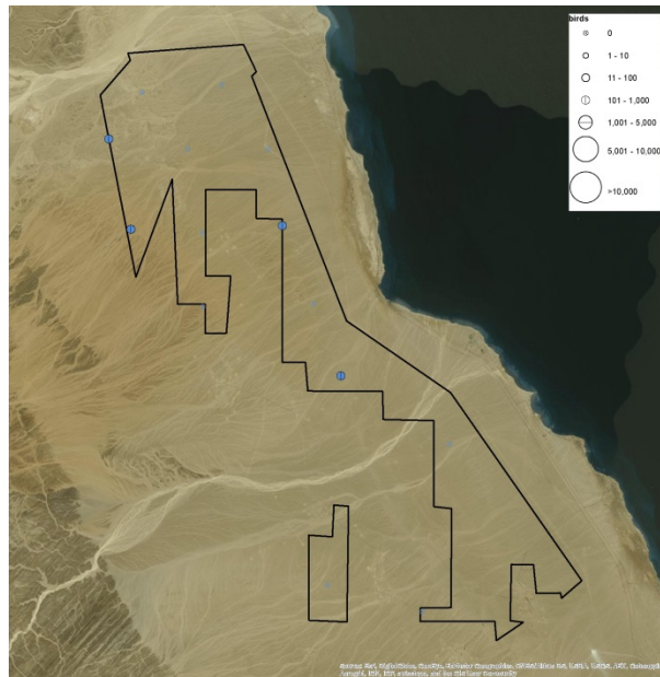
Number of birds (in abundance classes) registered within the study area in spring 2017
