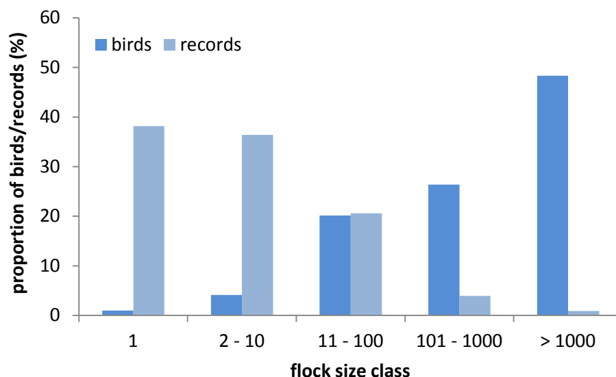
Figure 4.54: Relative abundance (proportion in %) of birds/records registered at distances of up to 2.5 km in different flock size classes in the Alfamar area in spring 2016
