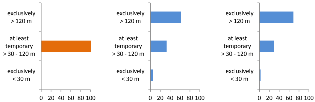
Relative abundance (percentage) of birds recorded at different altitude classes in the study area in autumn 2016 (n=1; left), spring 2016 (n=100; middle) and 2017 (n=472; right)
