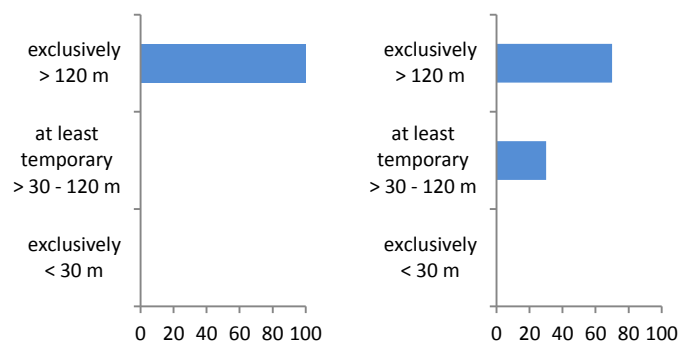
Relative abundance (percentage) of birds recorded at different altitude classes in the study area in spring 2016 (n=4; left) and 2017 (n=10; right)
