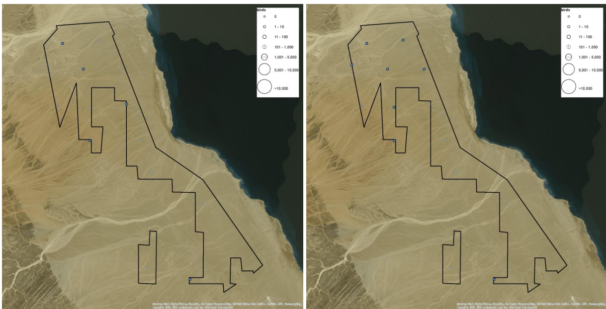
Number of birds (in abundance classes) registered within the study area in spring 2016 (left) and 2017 (right)
