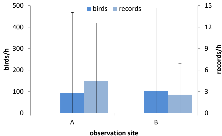
Figure 4.63: Comparison of migration rates during synchronized observation units at the two sites (A (n=154) and B (n=155)) in autumn 2015 (arithmetical mean and standard deviation over all observation units; sample size (i.e. no. of observation units) at each observation site is given in brackets)
