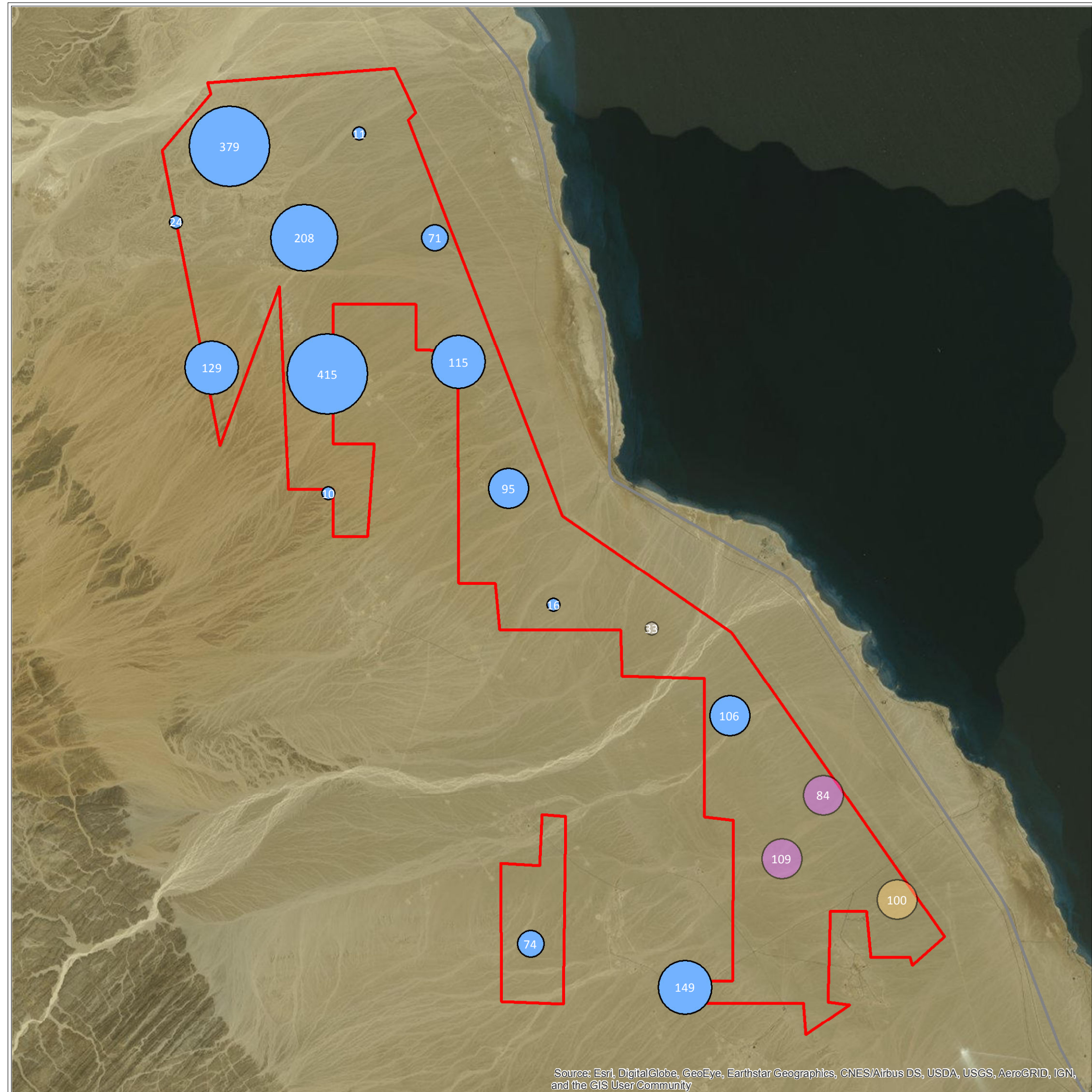
Map 4.4 Mean migration rate of target species (birds/h) obtained by different surveys in spring 2016
