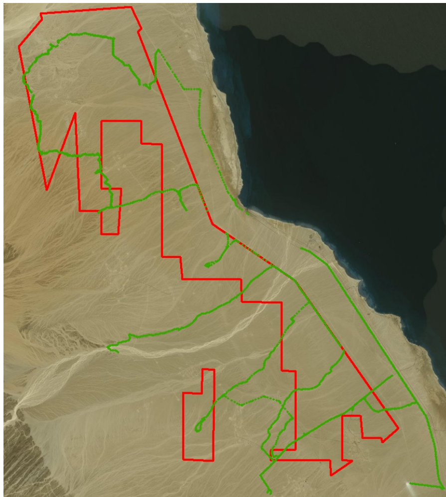
Figure 4.9: Main survey routes used during site visits for baseline surveys on habitats, flora and fauna
