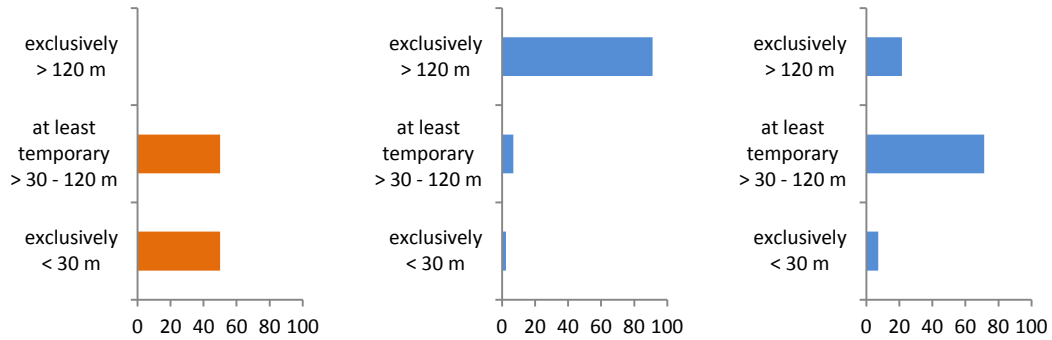
Relative abundance (percentage) of birds recorded at different altitude classes in the study area in autumn 2016 (n=2; left), spring 2016 (n=45; middle) and 2017 (n=14; right)
