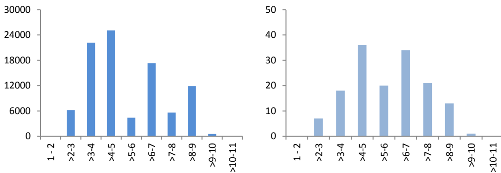
Number of birds (left) and records (right) registered in the study area at different hours after sunrise in spring 2016 (above) and 2017 (below) - no observations were conducted in early morning and evening
