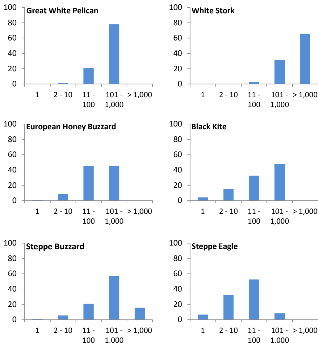
Figure 4.44: Relative abundance (proportion in %) of birds (blue) / records (light blue) of selected species registered at distances of up to 2.5 km in different flock size classes in spring 2017
