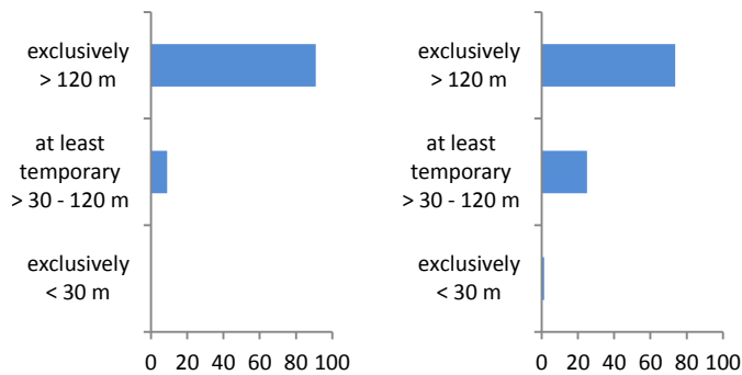
Relative abundance (percentage) of birds recorded at different altitude classes in the study area in spring 2016 (n=156; left) and 2017 (n=72; right)
