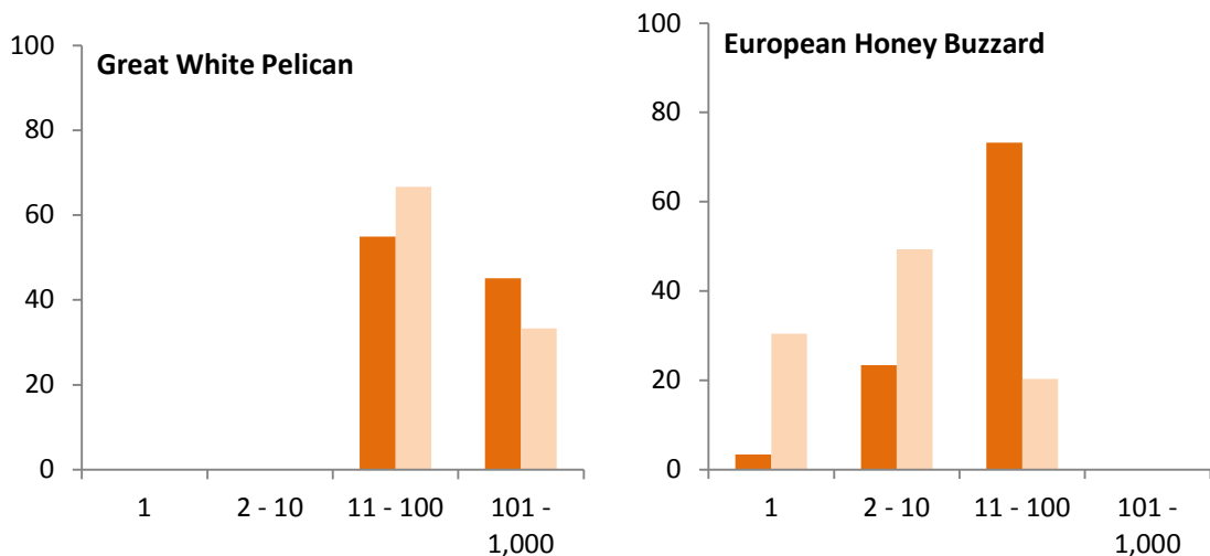
Figure 4.20: Relative abundance (proportion in %) of birds (orange) / records (light orange) of selected species in different flock size classes in the study period in autumn 2016
