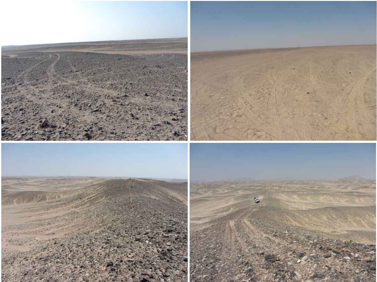
Figure 4.8: Typical surface material in the project area: levelled desert plain in the southern part of the project area (top) and hilly terrain in the north-western part of the project area (bottom)
