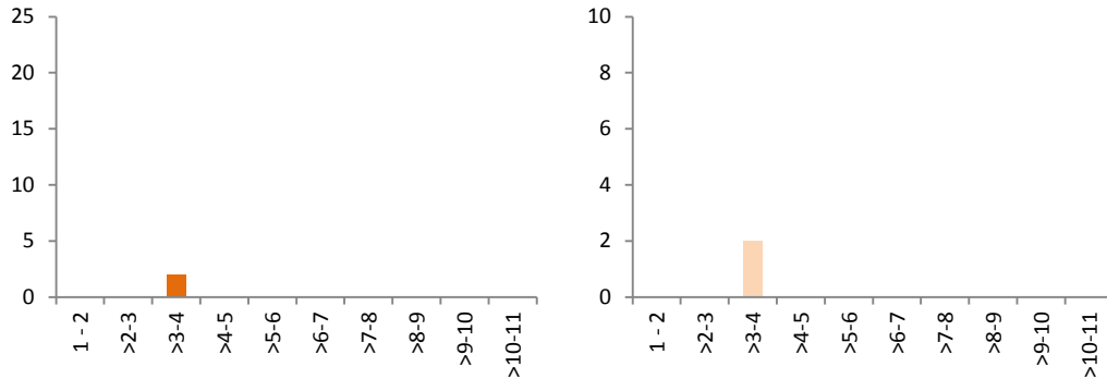
Number of birds (left) and records (right) registered in the study area at different hours after sunrise in autumn 2016 - no observations were conducted in early morning and evening
