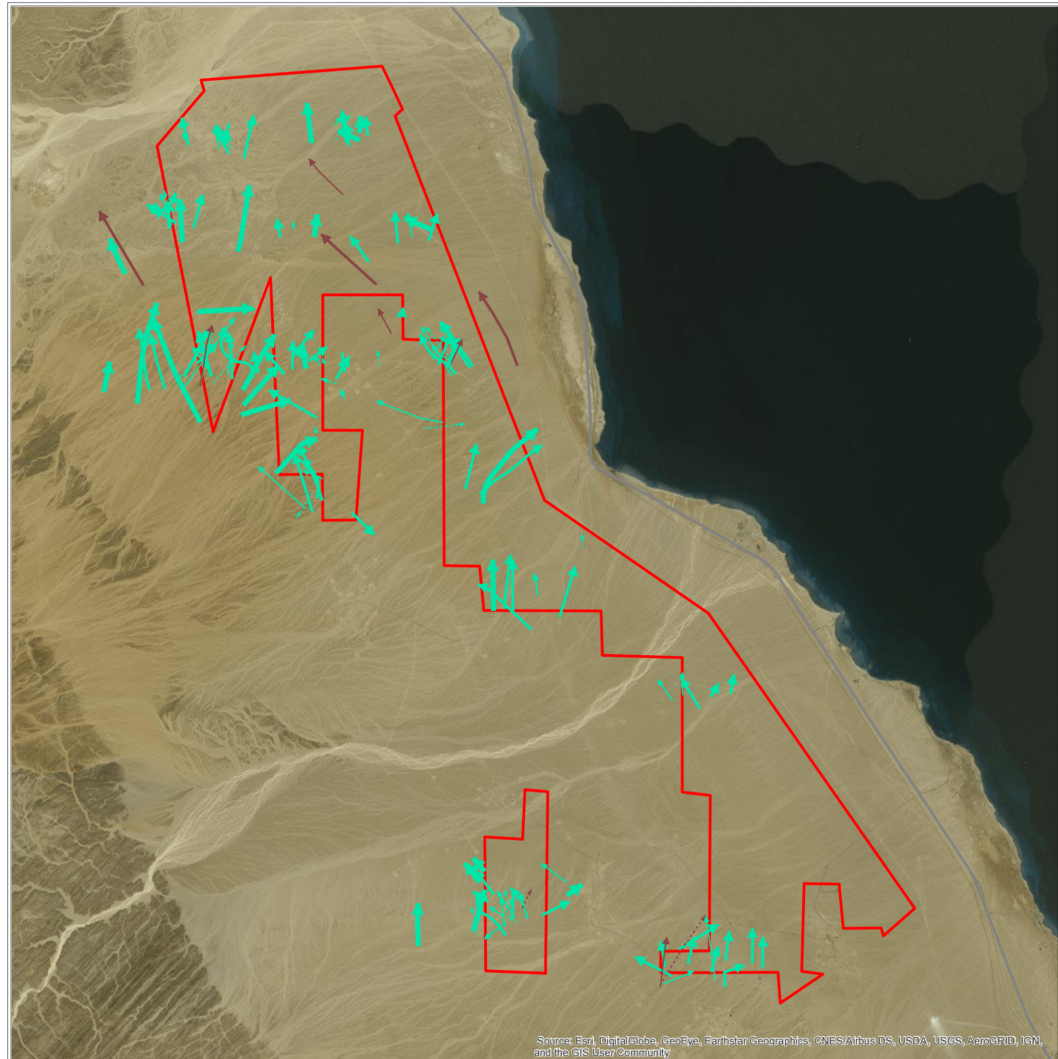
Map 4.8 Flight paths of Great White Pelican and White Stork during the study period in spring 2017
