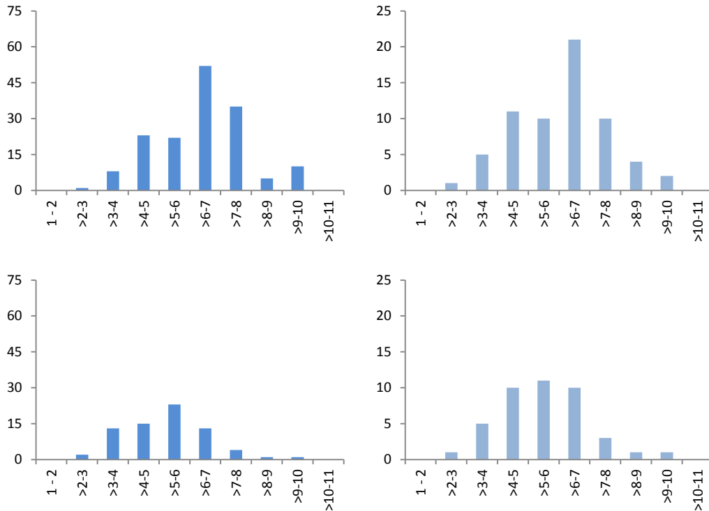
Number of birds (left) and records (right) registered at different hours after sunrise in the study area in spring 2016 (above) and 2017 (below) - no observations were conducted in early morning and evening
