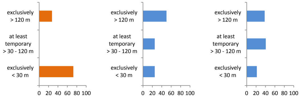
Relative abundance (percentage) of birds recorded at different altitude classes in the study area in autumn 2016 (n=11; left), spring 2016 (n=4; middle) and 2017 (n=42; right)
