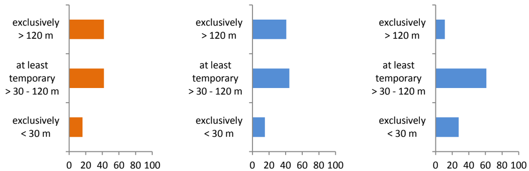
Relative abundance (percentage) of birds recorded at different altitude classes in the study area in autumn 2016 (n=31; left), spring 2016 (n=27; middle) and 2017 (n=36; right)
