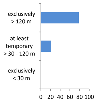
Relative abundance (percentage) of birds recorded at different altitude classes in the study area in spring 2017 (n=1,831)
