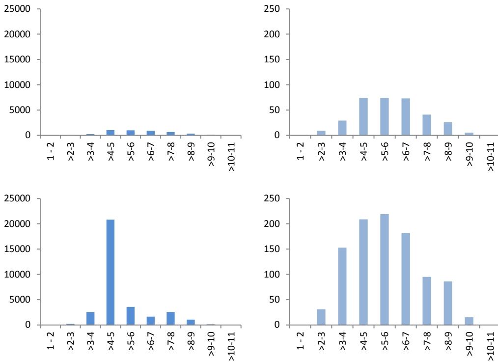
Number of birds (left) and records (right) registered in the study area at different hours after sunrise in spring 2016 (above) and 2017 (below) - no observations were conducted in early morning and evening
