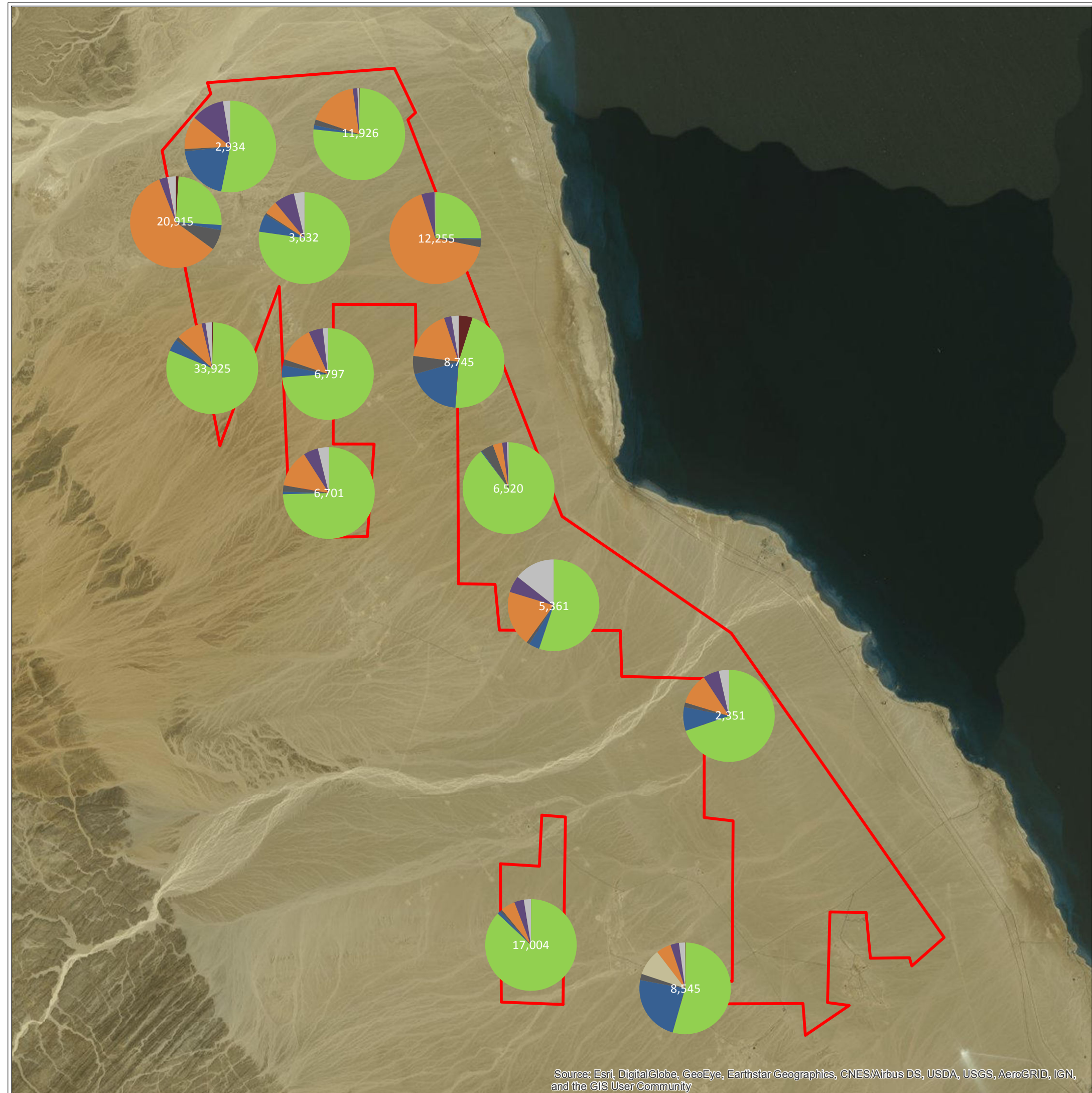
Map 4.7 Absolute number of birds and relative abundance of target species at each observation site in spring 2017
