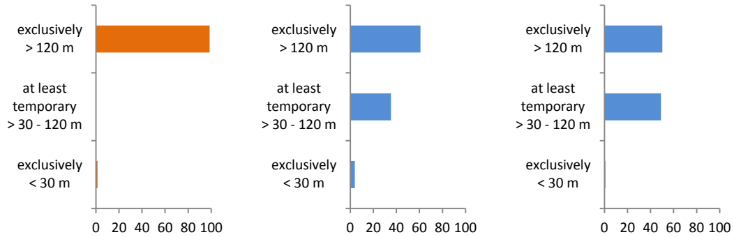
Relative abundance (percentage) of birds recorded at different altitude classes in the study area in autumn 2016 (n=636; left), spring 2016 (n=45,559; middle) and 2017 (n=93,199; right)
