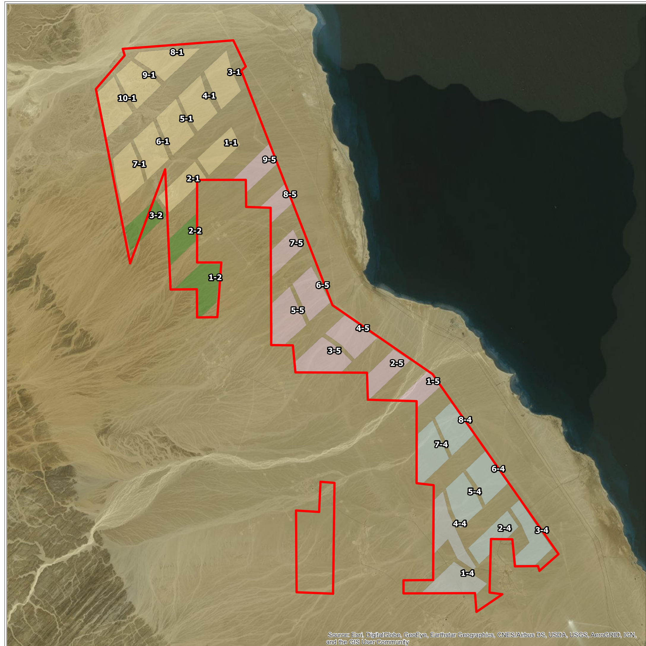
Map 5.1 Wind farm developments to be considered in the cumulative impact assessment for the project area
