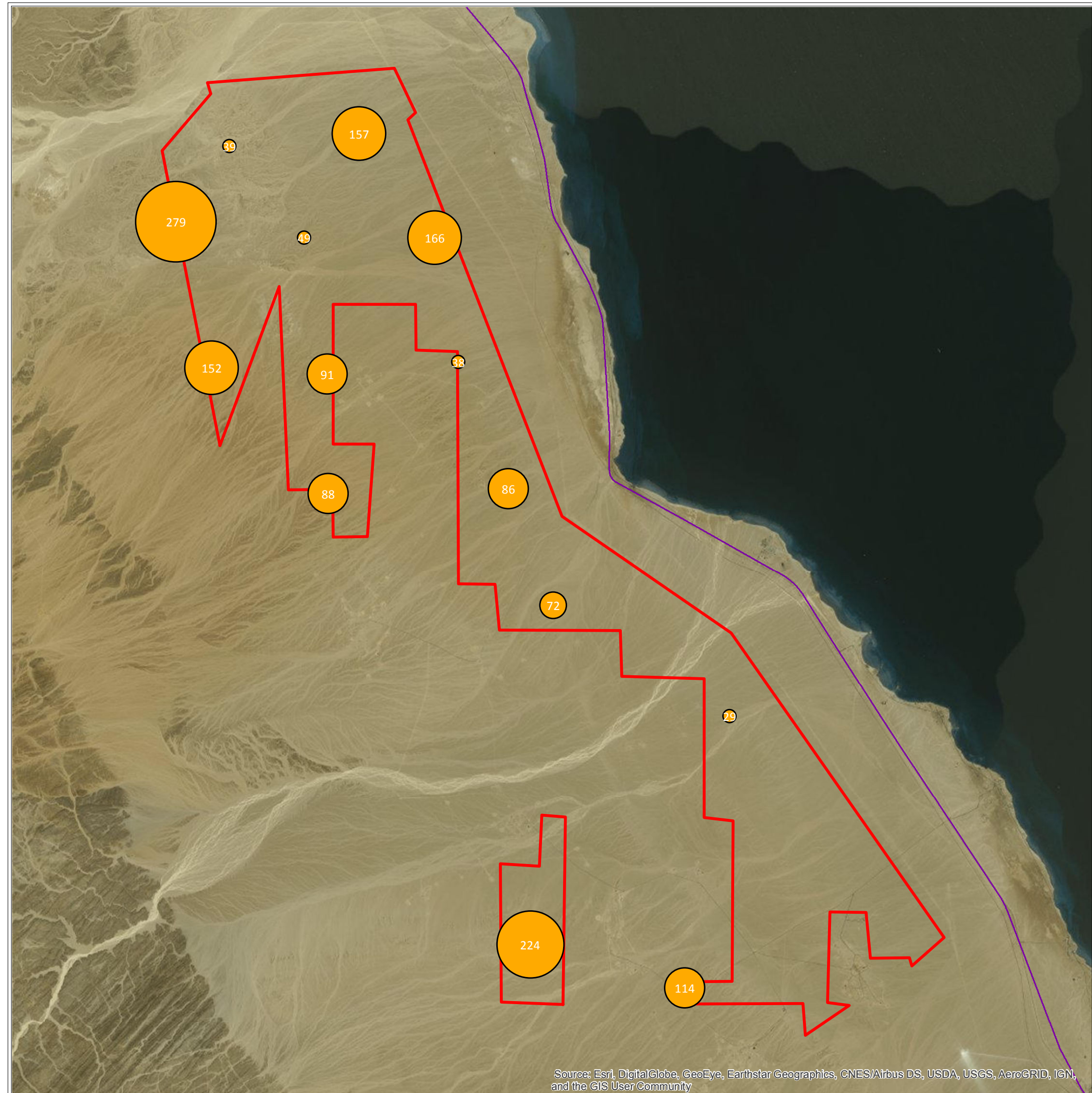
Map 4.6 Mean migration rate of target species (birds/h) obtained at observation sites in the project area in spring 2017
