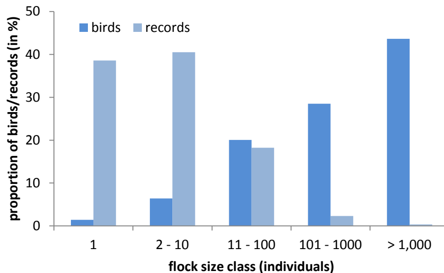
Figure 4.60: Relative abundance (proportion in %) of birds/records registered at distances of up to 2.5 km in different flock size classes in the ACWA area in spring 2016
