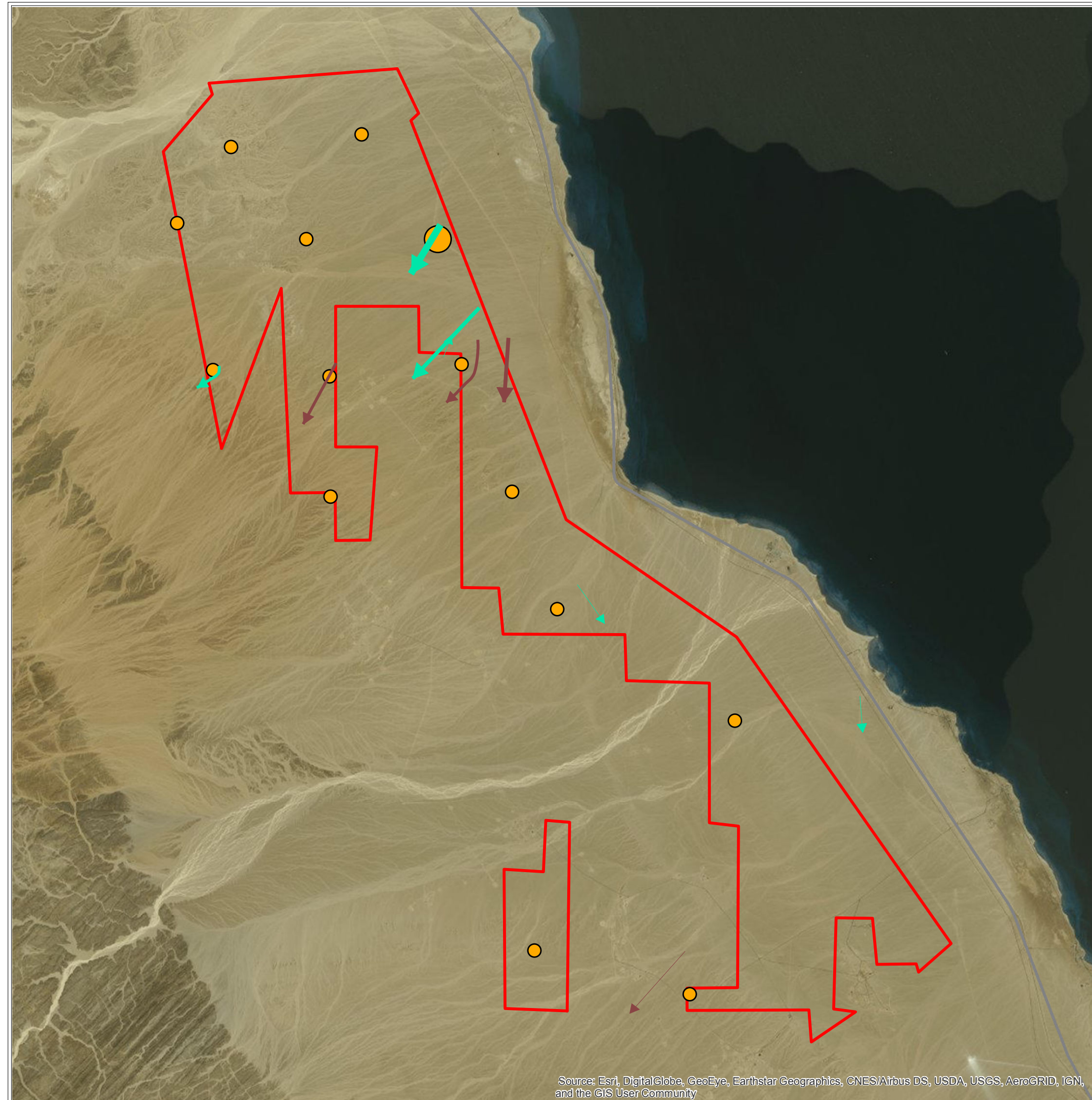
Map 4.3 Mean migration rate of target species (birds/h) at the 14 observation sites and flight paths of Great White Pelicans and White Storks in autumn 2016
