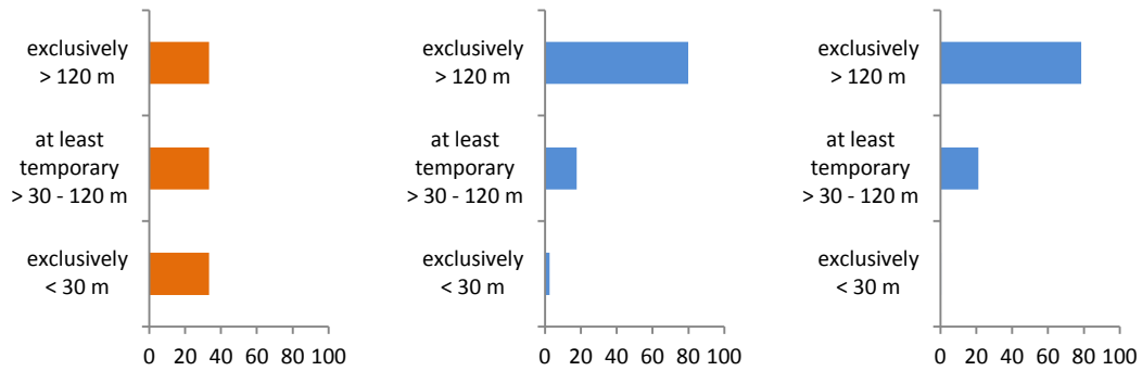
Relative abundance (percentage) of birds recorded at different altitude classes in the study area in autumn 2016 (n=3; left), spring 2016 (n=249; middle) and 2017 (n=4,740; right)
