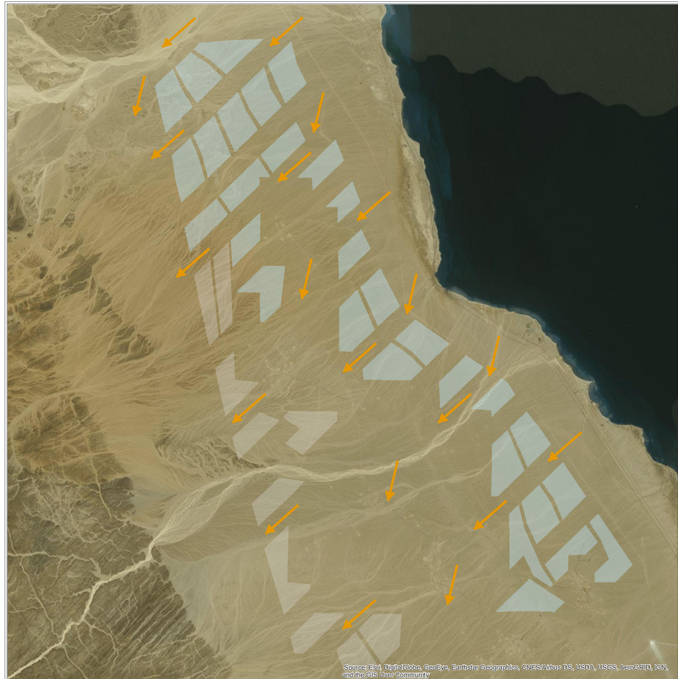
Map 5.2 Schematic illustration of likely flight paths of target species in autumn under the precondition of barrier effects caused by large wind farms
