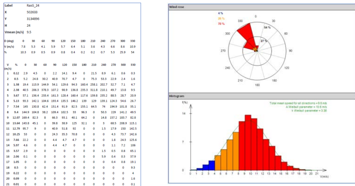
Figure 4.1: Ras Ghareb wind data summary, wind rose and wind speed distribution
